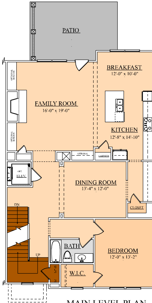
MAIN LEVEL PLAN
